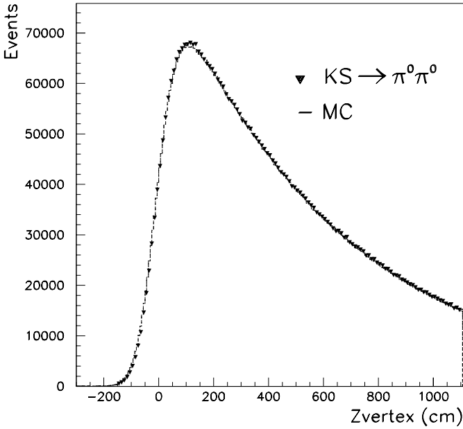
Fig. 9. Distribution of the reconstructed vertex position z_{vertex} of the K_S \rightarrow \pi^0\pi^0 candidates at the beginning of the decay volume. The origin of the z_{vertex} axis is set to the nominal AKS position
